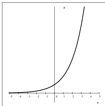
a > 1
