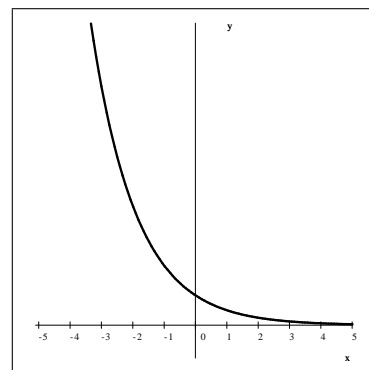
0 < a < 1
